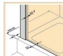
Installation on shower trays
