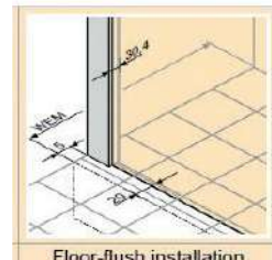
Floor-flush installation - scenario 001 WEM = Tray installation dim.
